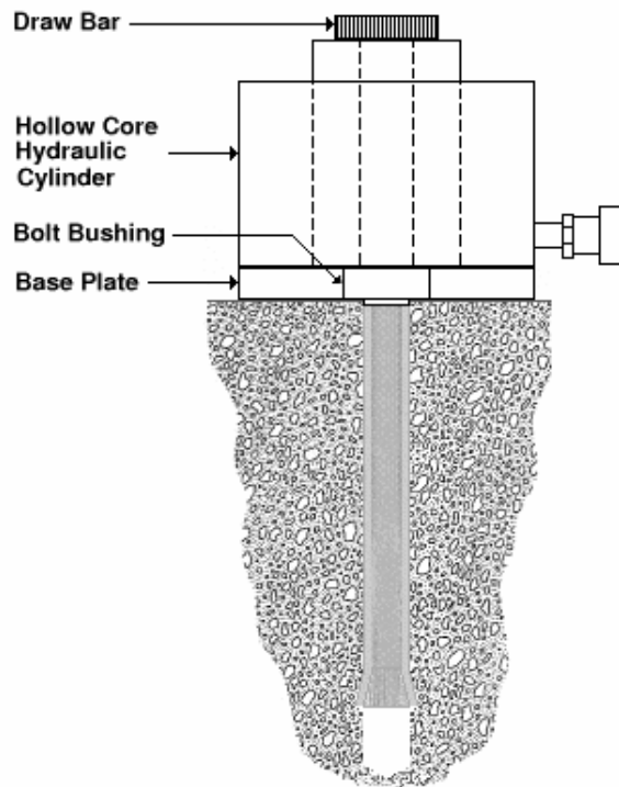
Hydraulic Setting Figure 4B
