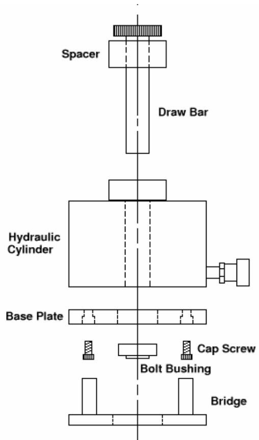
Hydraulic Assembly Figure 3
