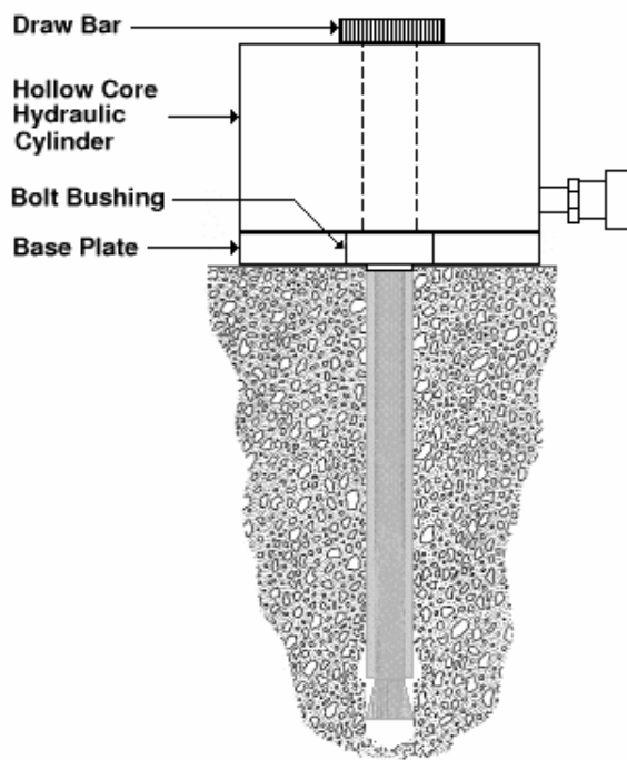
Hydraulic Setting Figure 4A
